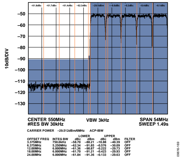
Figure 70. Mid Band Narrow-Band ACLR (Worse Side)
