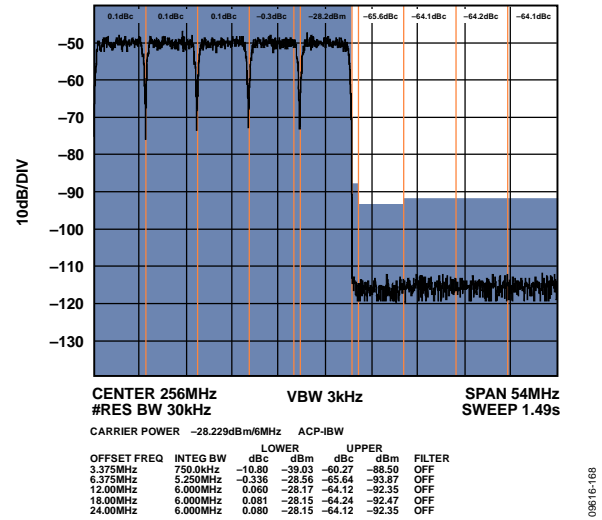
Figure 69. Low Band Narrow-Band ACLR
