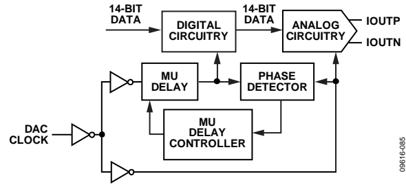
Figure 165. AD97339A Mu Delay Controller Block Diagram
