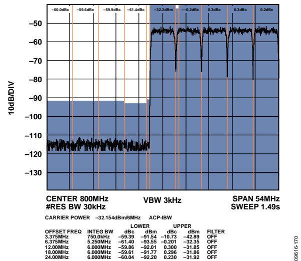
Figure 71. High Band Narrow-Band ACLR
