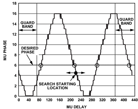
Figure 166. Typical Mu Phase Characteristic Plot at 2.4 GSPS
